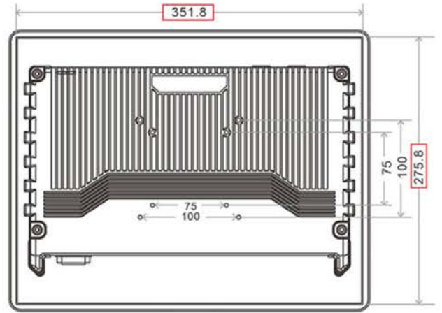
Back view
